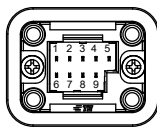
<Encoder Connector 핀 배열>
