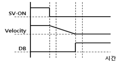
Free Run Stop 후 Hold
