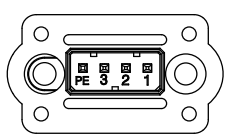
<Power Connector 핀 배열>
