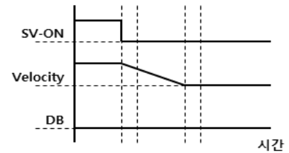
Free Run Stop 후 Release
