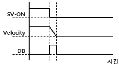
DB Stop 후 Release
