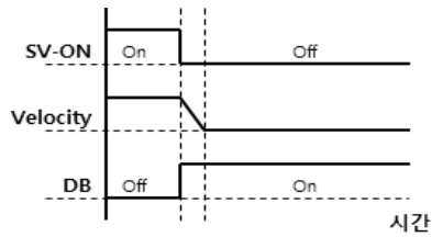
DB Stop 후 Hold
